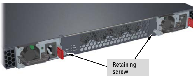
Figure 4-1. Fan tray assembly retaining screws
